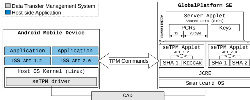
Figure 2: seTPM system architecture
