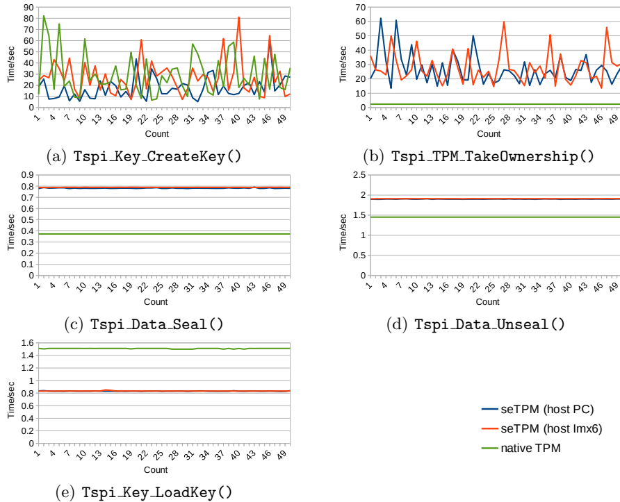
Figure 4: Evaluation of TPM 1.2 commands. The high-level TSPI commands internally invoke the associated TPM commands.
